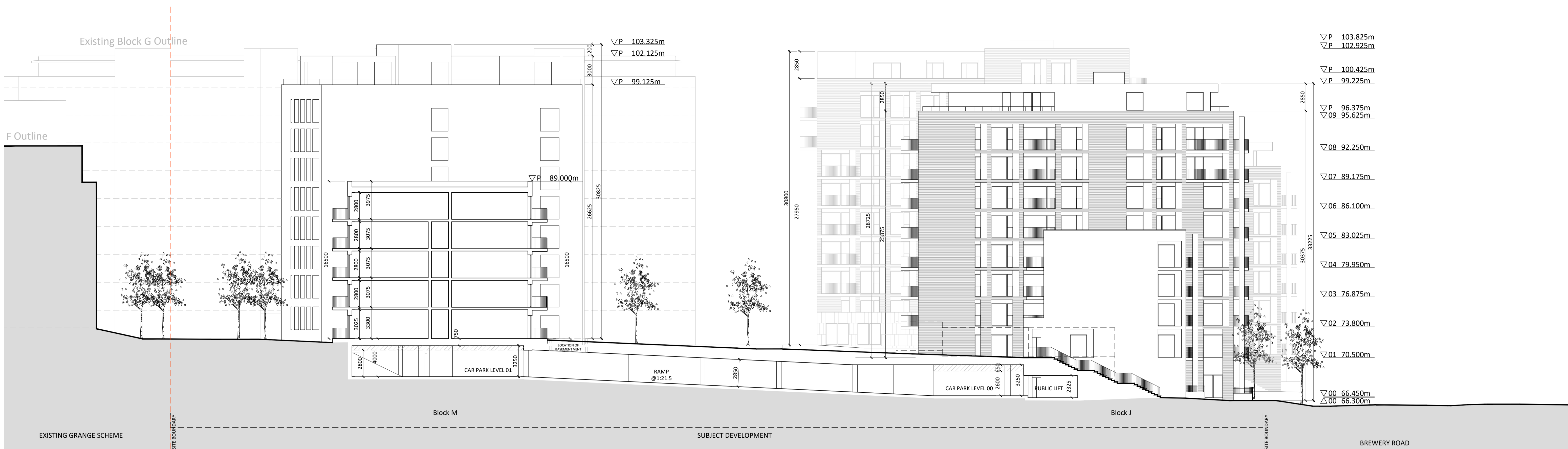
Section AA
